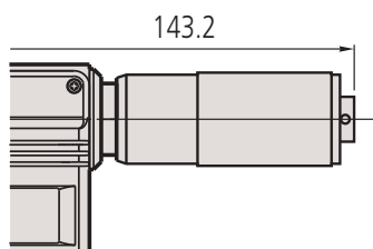
Friction thimble
