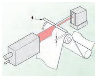
Measurement of film sheet thickness 1 Reference edge
