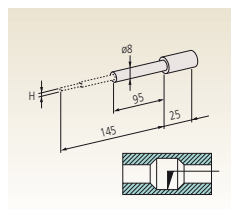
Arm for small-hole stylus CV-1000/2000
