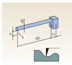
Arm Straight type CV-1000-2000
