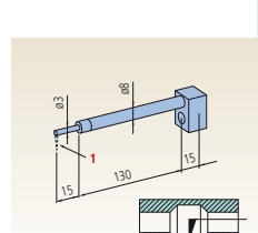
Arm for small-hole stylus
