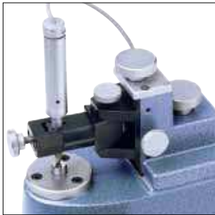
Calibrating a probe head.
