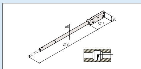
For small-hole stylus
