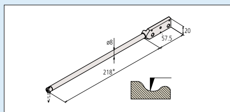
Straight type
